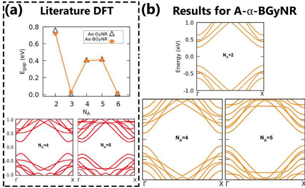
Figure 2.13: DFT and Tight-Binding calculations on A\alpha -BGyNR for Ab stacking (a) From top to bottom: Gap evolution of armchair monolayer and bilayer nanoribbons and band structures of N_A=4 and 5 of DFT calculations [81]. (b) Band structures of N_A=2, 4 , and 5 preserving the edges symmetry (here \Gamma X path stands for k_x \in [0, \pi/a] ).
